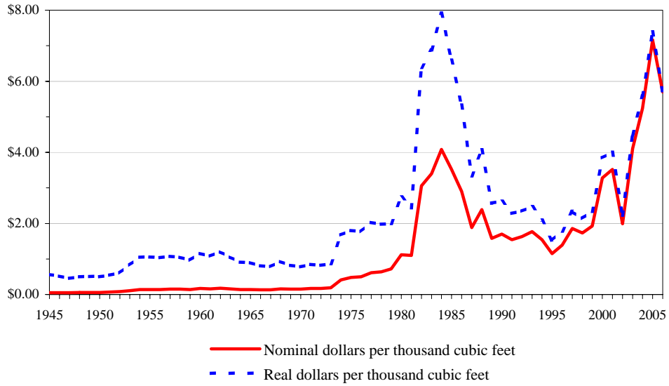
Figure 4.9 - Wellhead price of Natural Gas in Utah, 1945-2006
